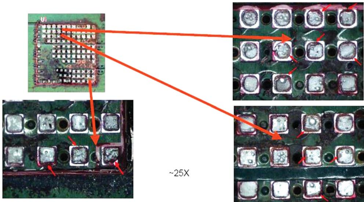
Figure 7. No Failure after 100,000 Cycles ( 50^{\circ}\text{C} - 100^{\circ}\text{C} )
